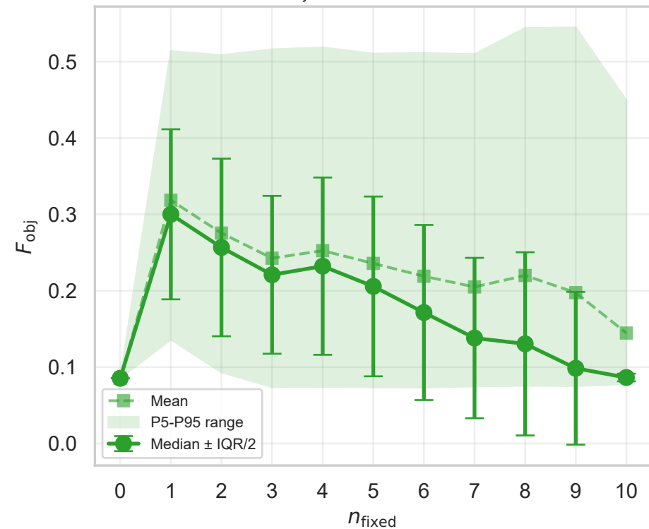
F_{\text{obj}} vs. Complexity
