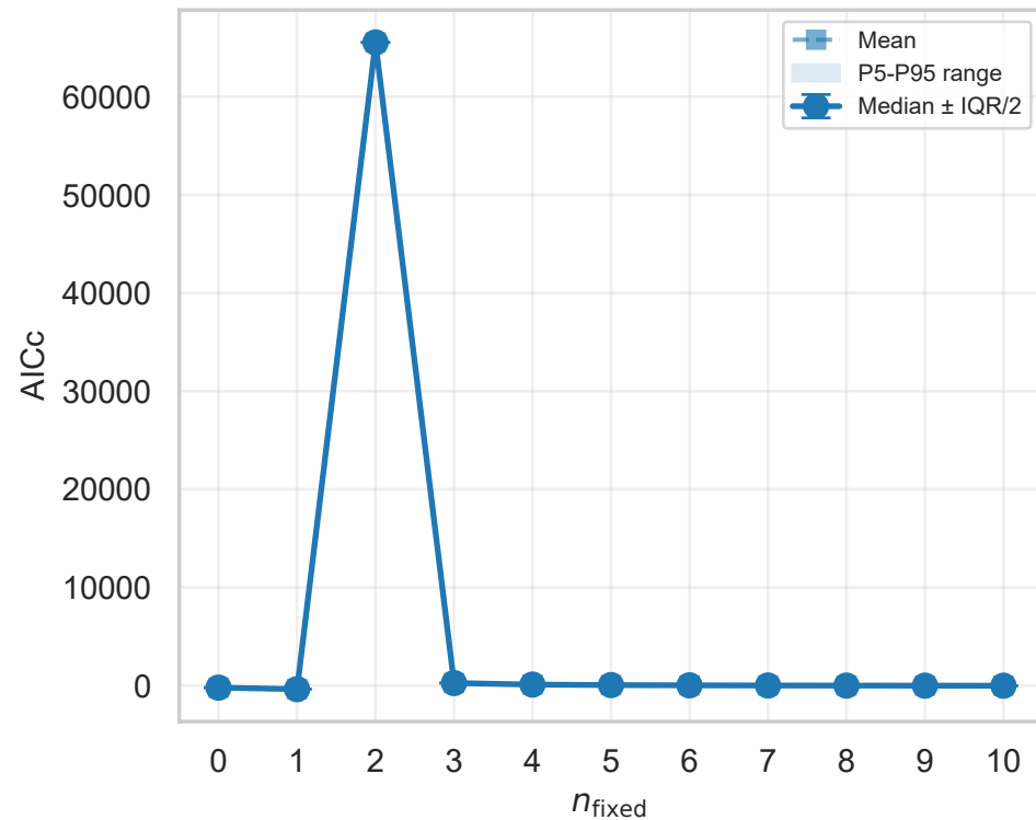
AICc vs. Complexity
