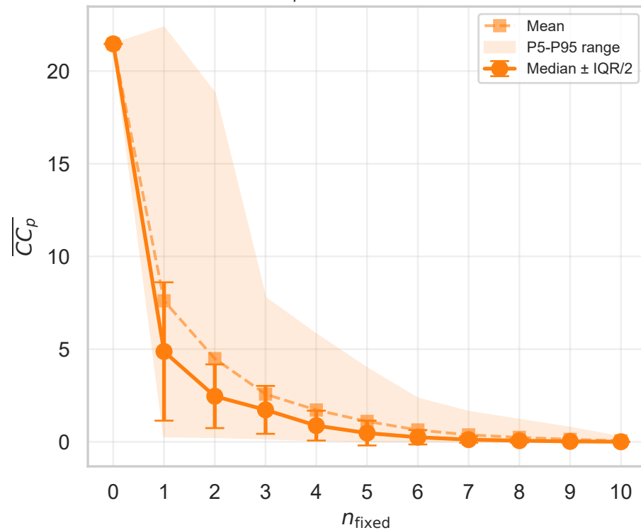
\overline{CC}_p vs. Complexity
